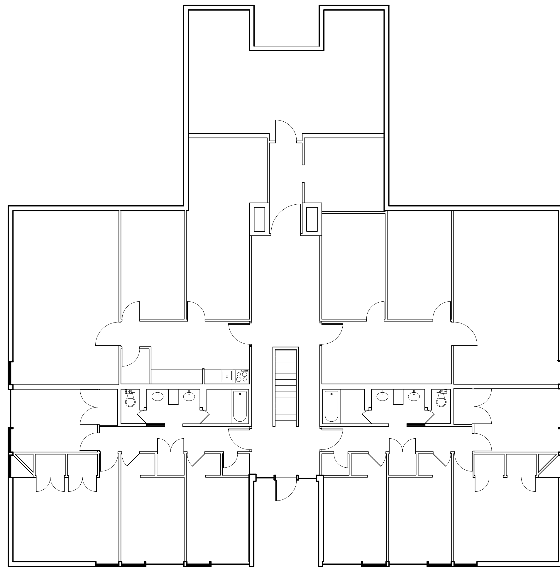
LOWER LEVEL
