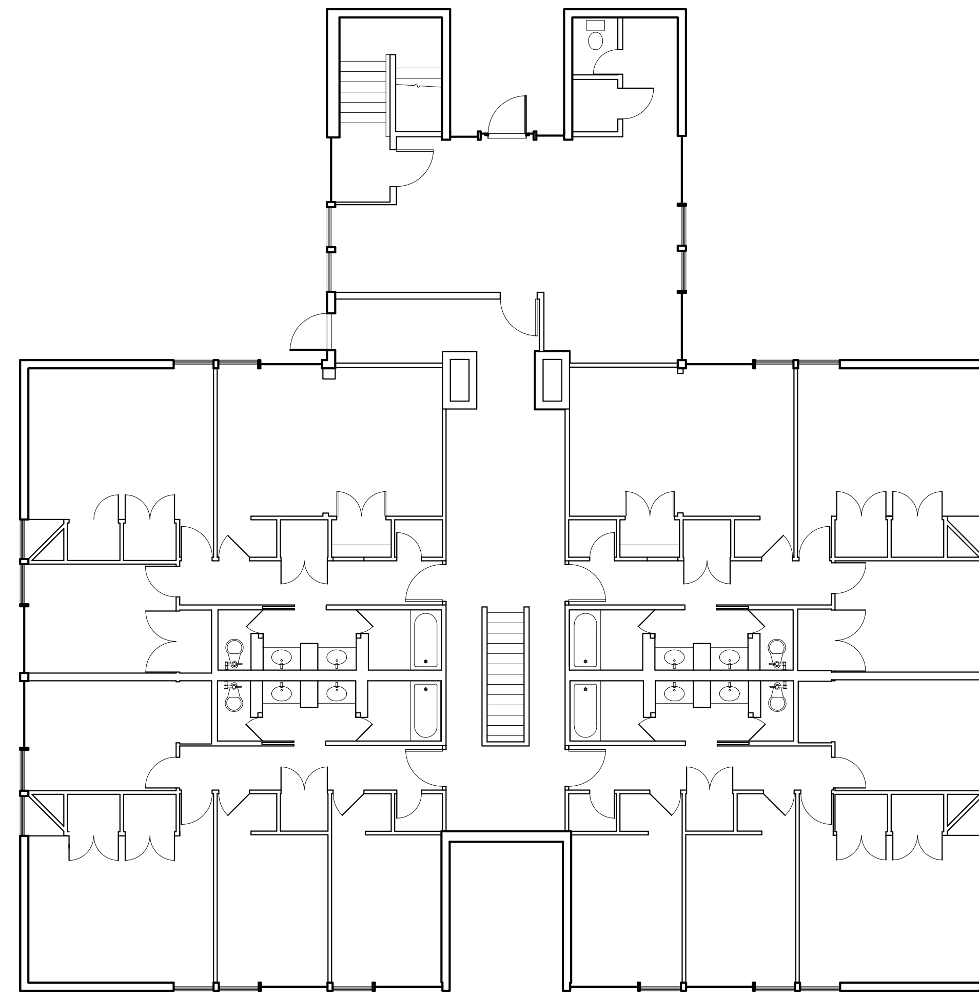
MAIN LEVEL
